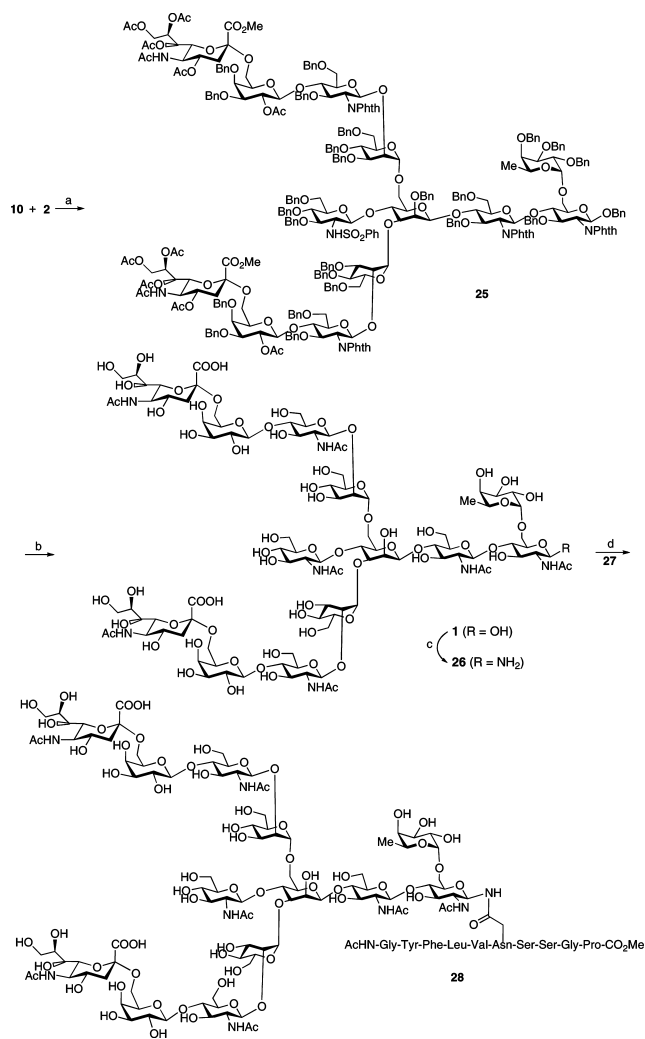
Scheme 4. Synthesis of Tridecasaccharide 1 and Glycopeptide 28 a
